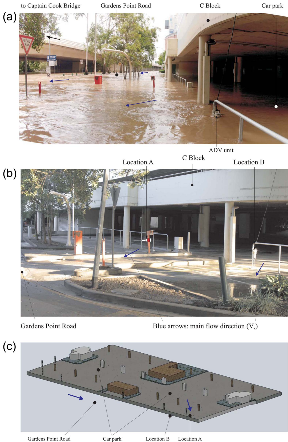
Figure 4. Field study in Gardens Point Road on 12–13 January 2011. The blue arrows show the main flow direction. (a) Inundated Gardens Point Road and C block building car park on 13 January 2011 at 11:40 (LT). Looking upstream at the flood flow. (b) Gardens Point Road and C block building car park on 14 January 2011 at 06:00. Note that both Gardens Point Road and C block building car park were cleaned up from any mud deposit during the night before. The ADV locations are highlighted. (c) Three-dimensional sketch of the C block building car park looking north.
