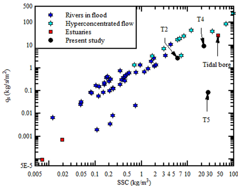
Figure 12. Suspended sediment flux q_s (kg s -1 m -2 ) as a function of the suspended sediment concentration SSC. Comparison between present data (periods T2, T4, and T5), observations in rivers during flood, and data in estuaries (Table 5).
